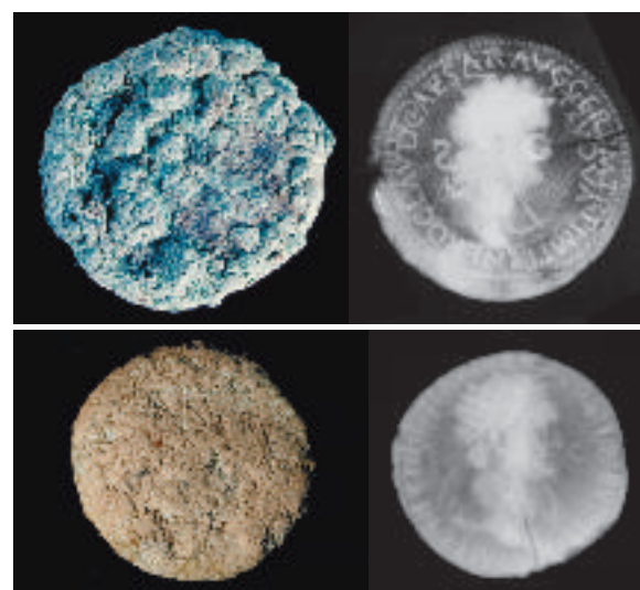
Fig 1 Coins can sometimes be dated from their X-radiographs. The two Roman coins, shown as excavated and their X-radiographs, are (upper) a sestertius of Nero dated AD 54–68 and (lower) a dupondius of Domitian dated AD 95–6.
