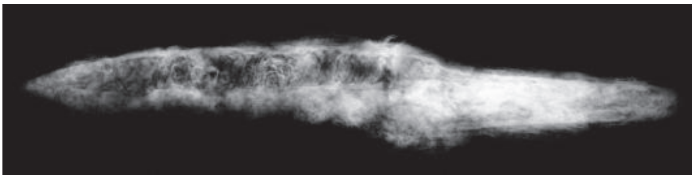
Fig 11 (below) Early medieval knife with pattern-welding in the back of the blade. Length: 178mm. Exposure: 3mA, 110kV, 60s, 0.45m FFD, Kodak Industrex MX.
