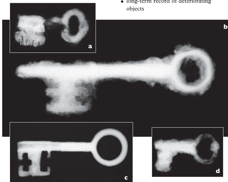
Fig 2 Good quality X-radiography reveals features of the four keys illustrated (2a–2d) that are obscured by corrosion and not visible even under magnification. Three of the four (2a, 2b, 2d) are plated, two (2c, 2d) have decorative mouldings at the neck, one (2c) being finely grooved. The nature of the key bit is clarified on three of the examples. 2a has multiple clefts, 2d has opposing channelled clefts. 2b is a door key as, having a symmetrical bit, it could be used from either side of the lock. It has a solid stem projecting beyond the end of the bit and a collar above. The stem of 2c is hollow and the piped stem fitted over a locating pin in the lock. Length of keys: 2a, 65mm; 2b, 175mm; 2c, 98mm; 2d, 58mm.
